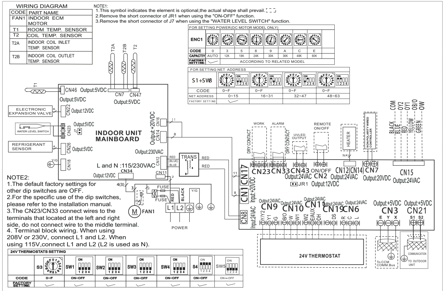
Fig. 13 —Wiring Diagram Sizes 30K, 36K, 48K, 60K
