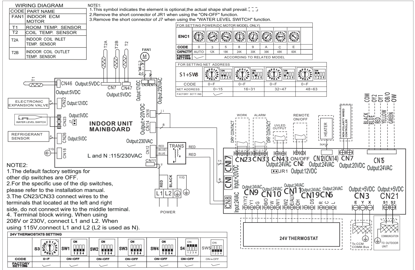
Fig. 12 — Wiring Diagram Sizes 18K, 24K
