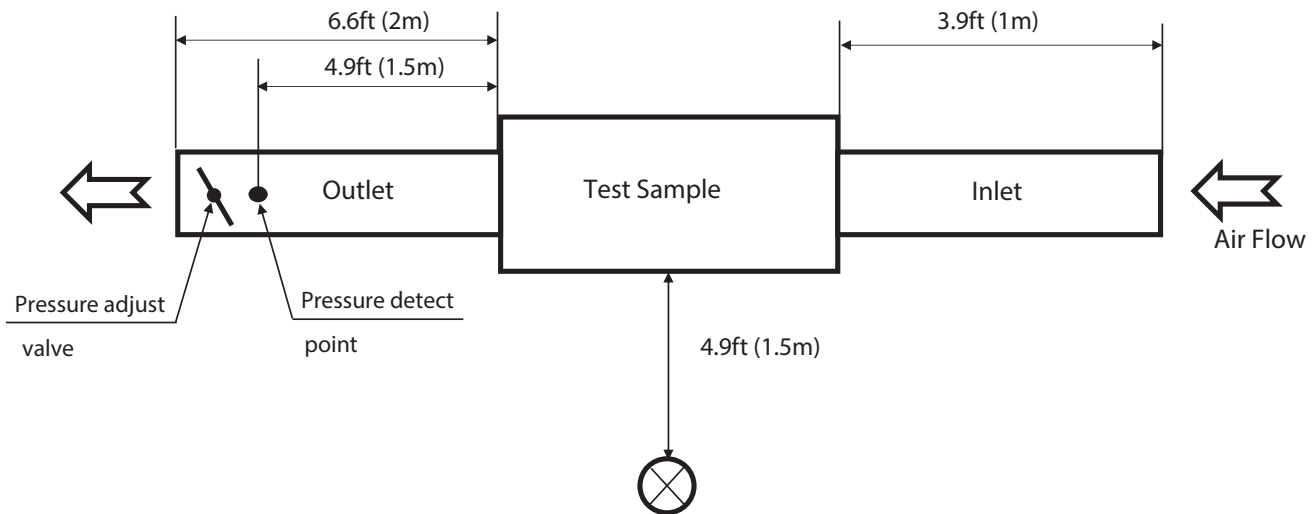
Fig. 11 — Sound Pressure Testing Method
