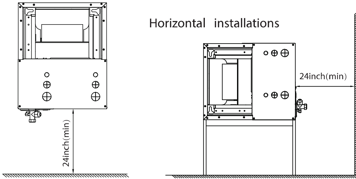
Fig. 7 — Clearances
