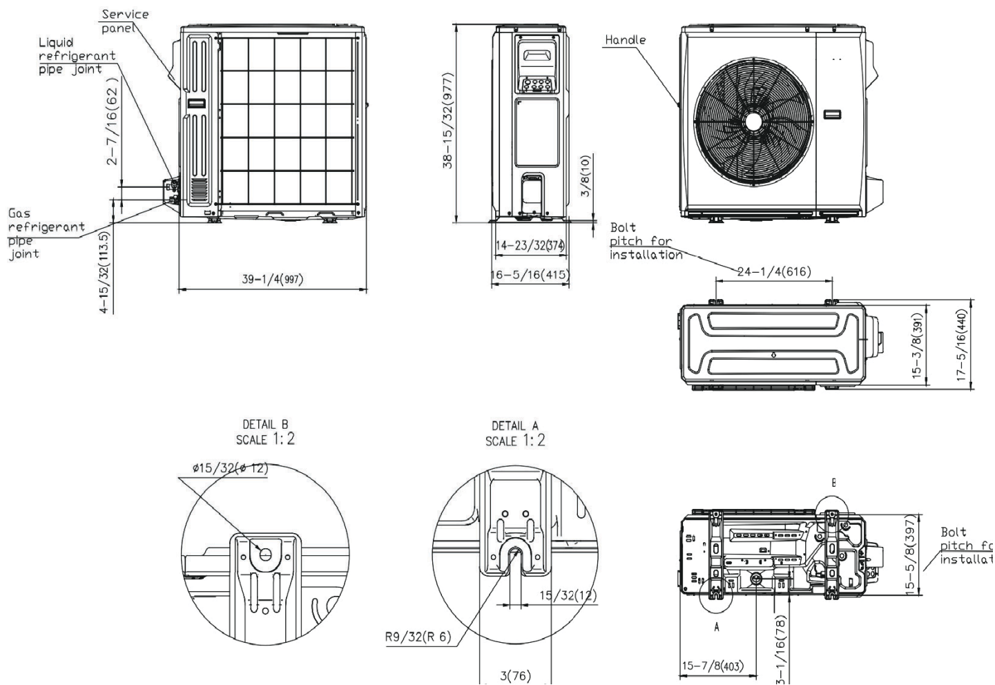
Fig. 5 – Sizes 48/60K
