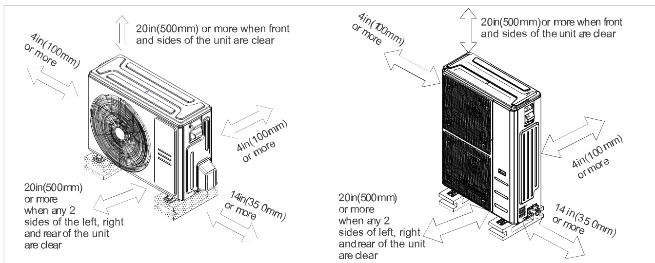
Fig. 6 – Clearances
