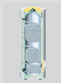
Stainless steel, dual-coil DHW tank
